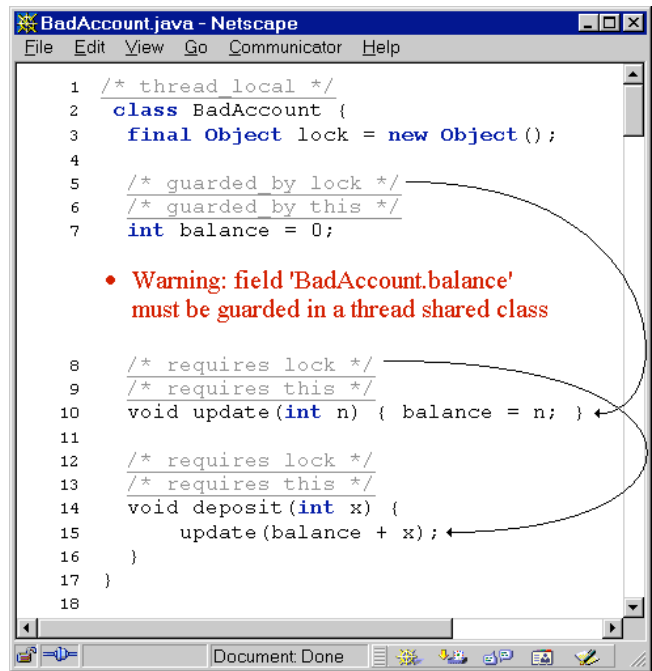
Figure 4: Screen shot showing the Houdini/rcc user interface for the broken BadAccount class. The overlaid arrows indicate where two of the hyper-links are pointing.
